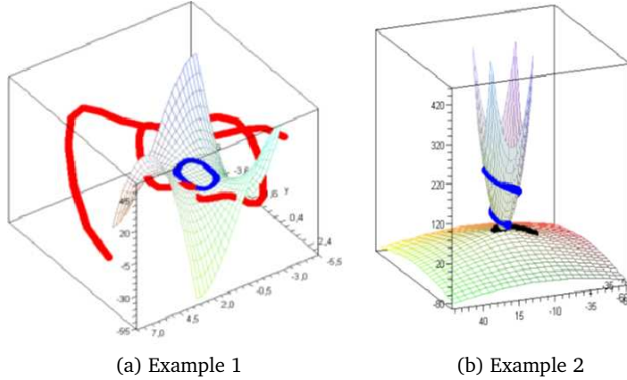
Figure 1: Special Involute-Evolute Partner D-curves.
